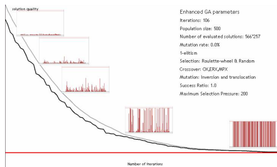
Figure 5: The distribution of essential genetic information when using the enhanced selection concept considering the ch130 benchmark TSP without mutation.
