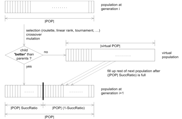
Figure 1: Flowchart of Offspring Selection
